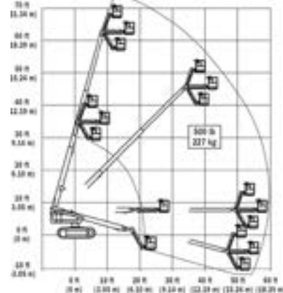
JLG 660SJC
