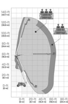
DIESEL 1250AJP
