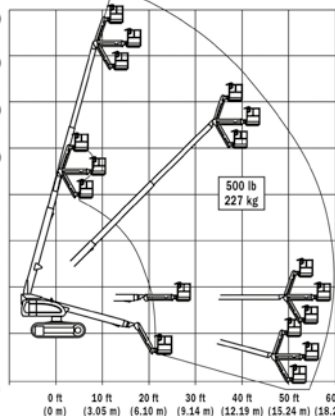
JLG 660SJC
