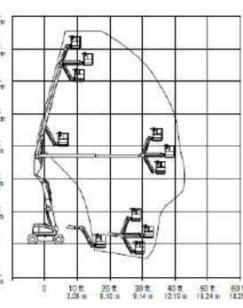
DIESEL 600AJ
